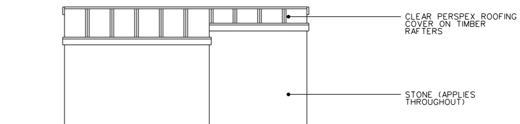
EXISTING REAR ELEVATION (NORTH)
